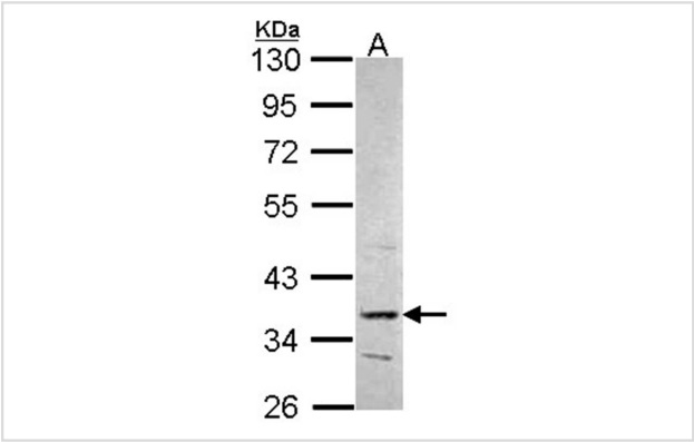
Sample (30 ug of whole cell lysate) A: Hep G2 10% SDS PAGE PRPS2 antibody diluted at 1: 1000
