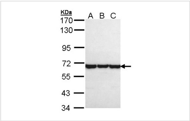
Sample (30 ug of whole cell lysate) A: A431 B: H1299 C: Hela 7.5% SDS PAGE Primary antibody diluted at 1: 1000
