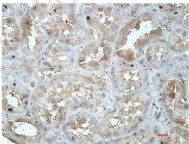
Immunohistochemical staining of formalin-fixed paraffin-embedded human kidney staining with anti-C14ORF28 antibody at a dilution of 1/100
