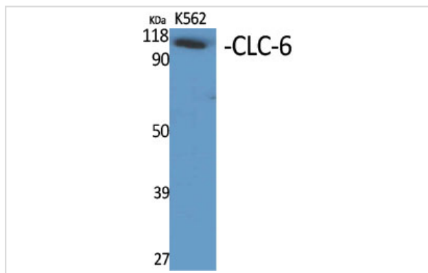
Western Blot analysis of K562 cells using CLC-6 Polyclonal Antibody
