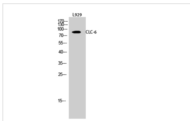
Western Blot analysis of L929 cells using CLC-6 Polyclonal Antibody
