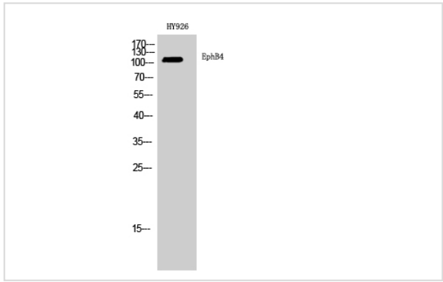
Western Blot analysis of HY926 cells using EphB4 Polyclonal Antibody
