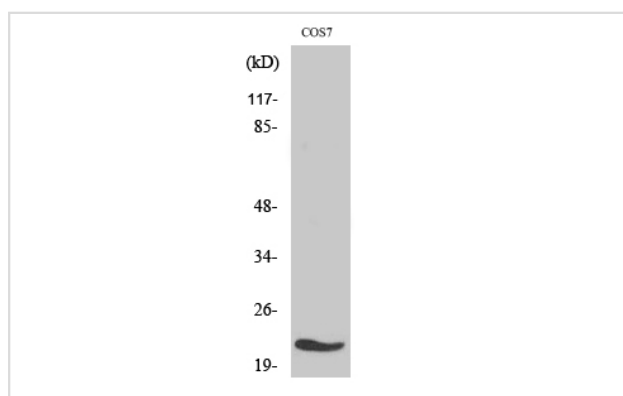
Western Blot analysis of COS7 cells using MRP-L11 Polyclonal Antibody
