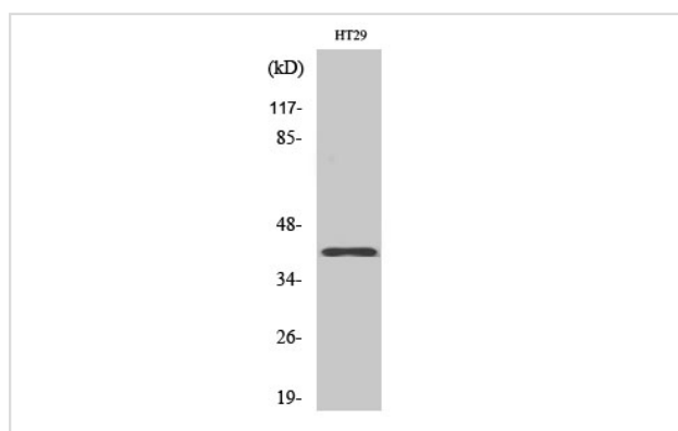
Western Blot analysis of HT29 cells using Olfactory receptor 8S1 Polyclonal Antibody
