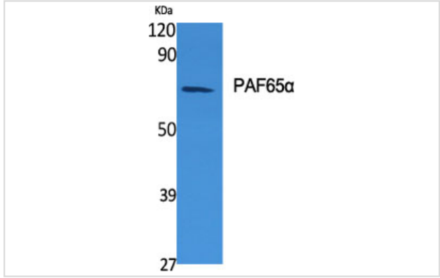
Western Blot analysis of various cells using PAF65α Polyclonal Antibody
