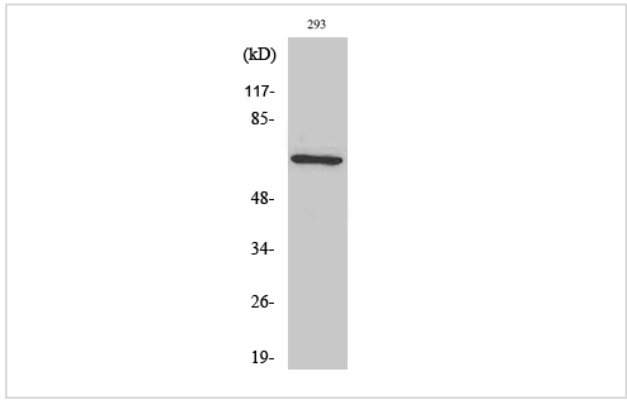
Western Blot analysis of 293 cells using PAF65α Polyclonal Antibody
