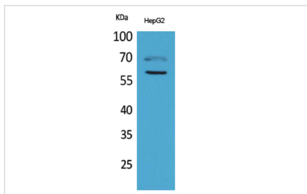
Western Blot analysis of HepG2 cells using HEXA Polyclonal Antibody
