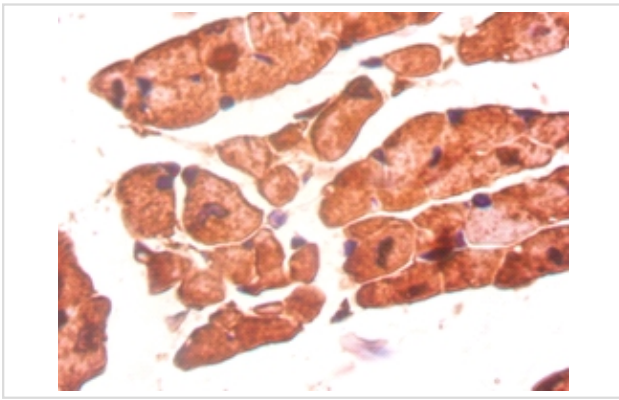
Immunohistochemical analysis of paraffin-embedded mouse heart using #42083 at dilution of 1:100.
