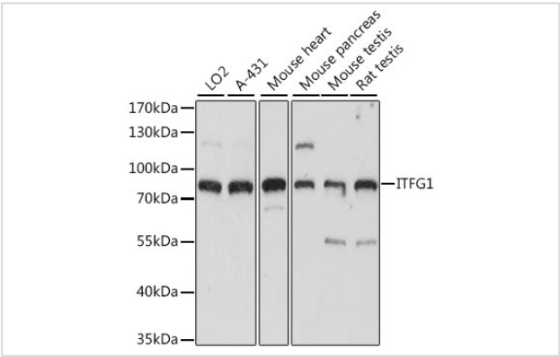
Western blot analysis of extracts of various cell lines, using ITFG1 at 1:1000 dilution.
