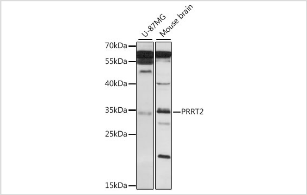
Western blot analysis of extracts of various cell lines, using PRRT2 at 1:1000 dilution.
