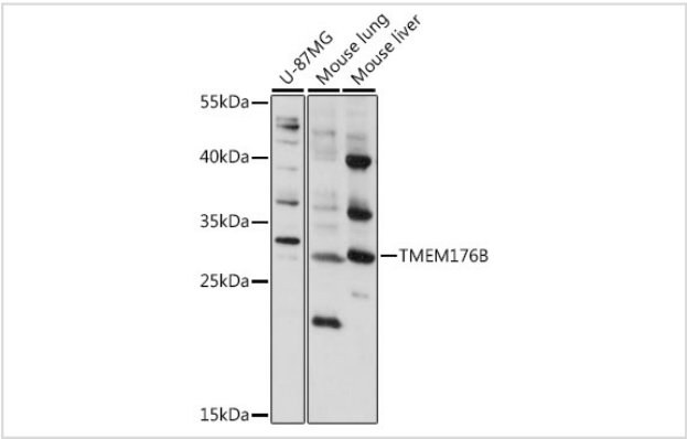
Western blot analysis of extracts of various cell lines, using TMEM176B at 1:1000 dilution.
