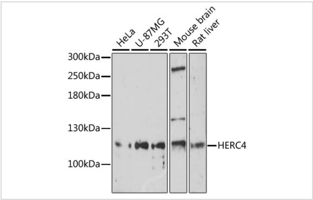
Western blot analysis of extracts of various cell lines, using HERC4 at 1:1000 dilution.
