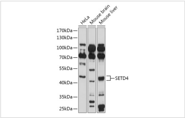
Western blot analysis of extracts of various cell lines, using SETD4 at 1:1000 dilution.
