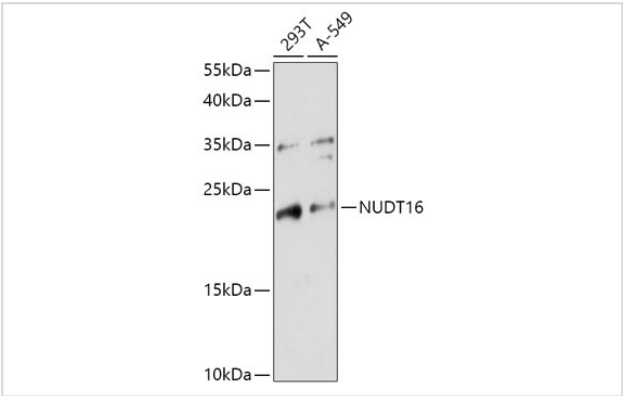
Western blot analysis of extracts of various cell lines, using NUDT16 at 1:1000 dilution.
