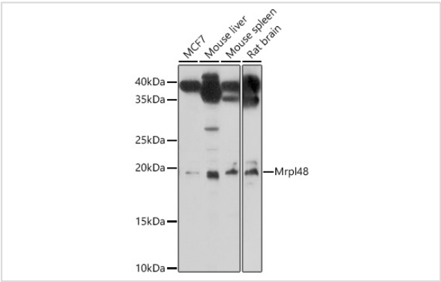
Western blot analysis of extracts of various cell lines, using Mrpl48 at 1:1000 dilution.
