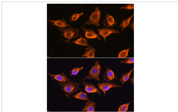
Immunofluorescence analysis of L929 cells using ZCCHC11 Rabbit pAb.
