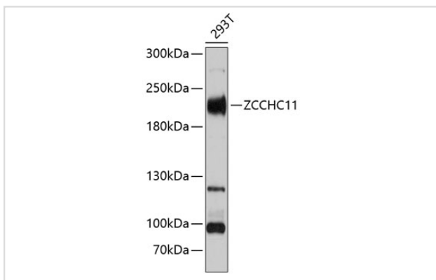
Western blot analysis of extracts of 293T cells, using ZCCHC11 Antibody.
