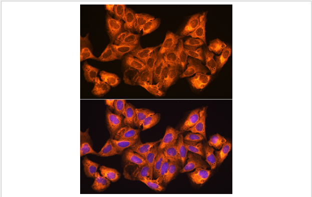
Immunofluorescence analysis of U2OS cells using ZCCHC11 Rabbit pAb.
