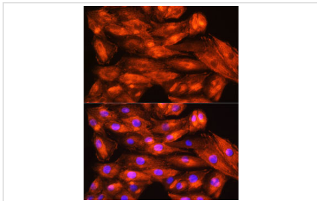
Immunofluorescence analysis of H9C2 cells using ZCCHC11 Rabbit pAb.
