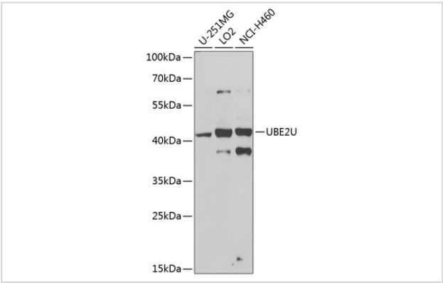
Western blot analysis of extracts of various cell lines, using UBE2U at 1:1000 dilution.
