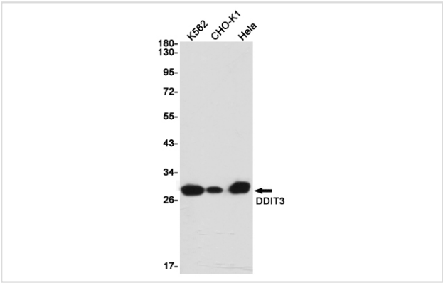
Western blot detection of DDIT3 in K562,CHO-K1,HeLa cell lysates using DDIT3 Rabbit mAb(1:1000 diluted).Predicted band size:19KDa.Observed band size:27KDa.
