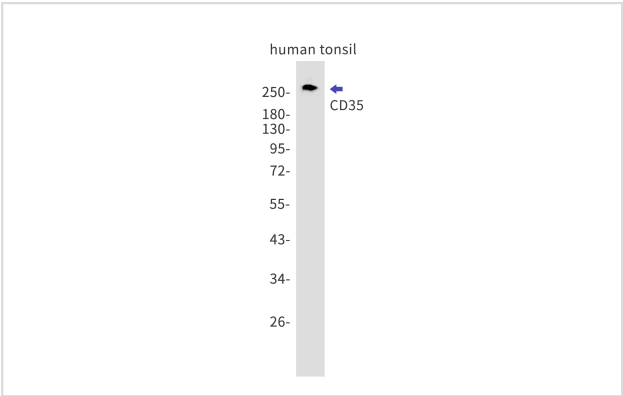
Western blot detection of CD35 in human tonsil lysates using CD35 antibody. Predicted band size: 224kDa. Observed band size: 280kDa.
