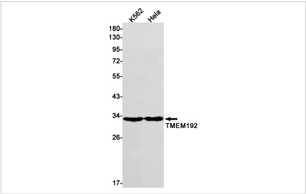
Western blot detection of TMEM192 in K562,HeLa cell lysates using TMEM192 Rabbit mAb(1:1000 diluted).Predicted band size:31kDa.Observed band size:31kDa.
