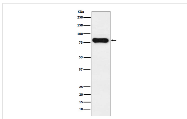
Western blot analysis of IGH expression in Human tonsil cell lysate.
