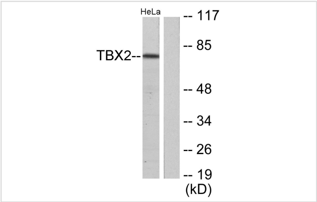
Western blot analysis of lysates from HeLa cells, using TBX2 Antibody. The lane on the right is blocked with the synthesized peptide.
