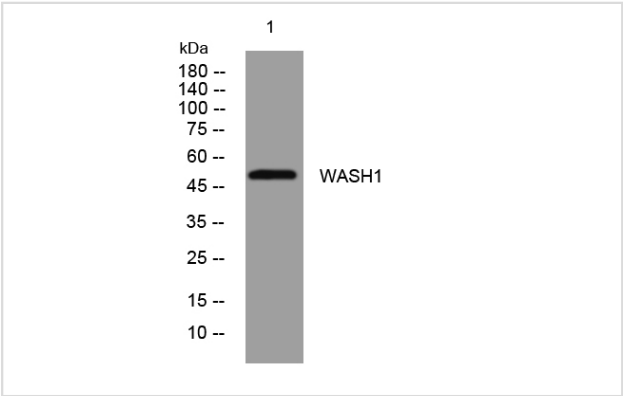
Western blot analysis of lysates from U2OS cells using WASH1 antibody at 1:1000.
