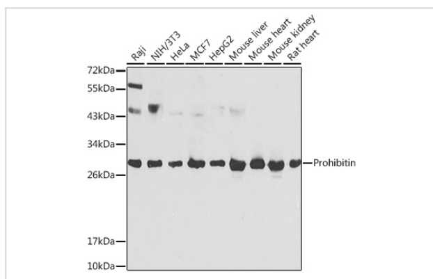
Western blot analysis of extracts of various cell lines, using Prohibitin antibody.
