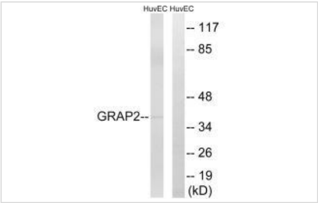
Western blot analysis of extracts from HuvEc cells, using GRAP2 antibody #34707.
