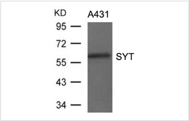
Western blot analysis of extracts from A431 cells using SYT Antibody #21438.
