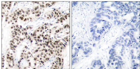
Immunohistochemical analysis of paraffin-embedded human breast carcinoma tissue using Myc(Ab-58) Antibody #21034(left) or the same antibody preincubated with blocking peptide(right).
