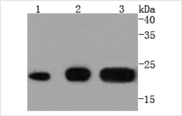
Western blot analysis of CD81 on different lysates using anti-CD81 antibody at 1/1,000 dilution. Positive control: Lane 1: JAR Lane 2: PC-12 Lane 3: K562
