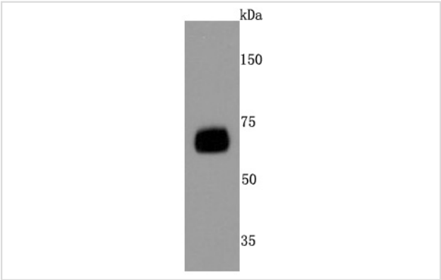
Western blot analysis of CD73 on A431 cells lysates using anti-CD73 antibody at 1/500 dilution.
