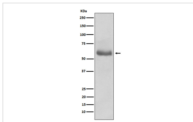
Western blot analysis of Oct-2 expression in Ramos cell lysate.
