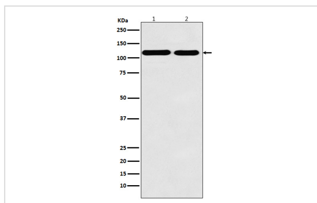
Western blot analysis of Matrin 3 expression in (1) HEK293 cell lysate; (2) PC12 cell lysate.
